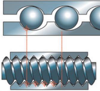
The depiction above illustrates the limited number of contact points in a ball screw compared to the contact points in a planetary roller screw design.
